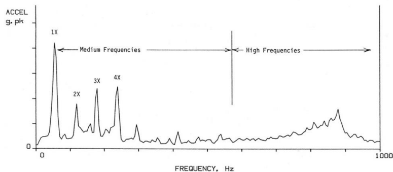
Fig 2. An example FFT spectrum of common machinery vibration.
