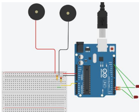
Fig. 1. Experimental setup of measuring device
