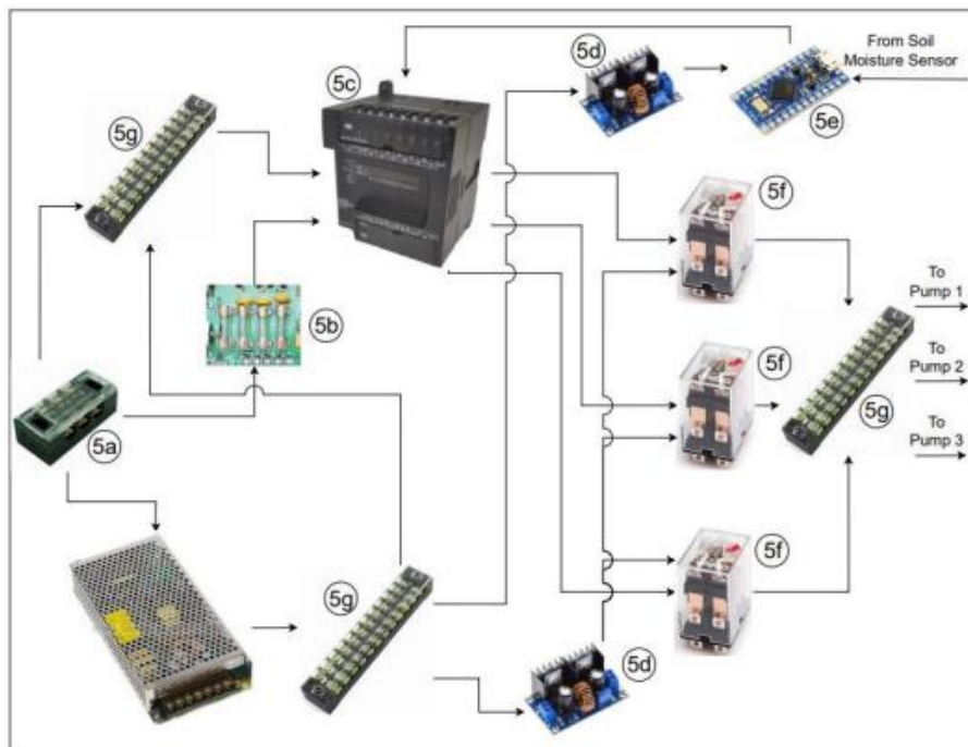
Fig 2. Soil moisture controller concept schematic
