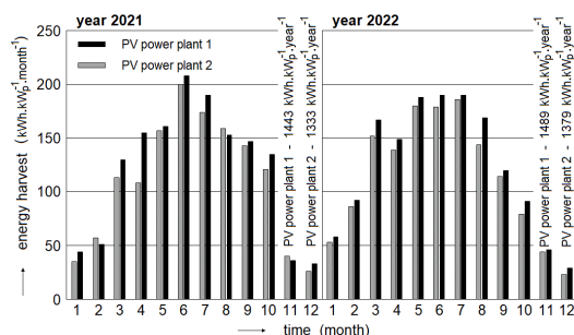
Fig. 2 Electricity production during the last two years
