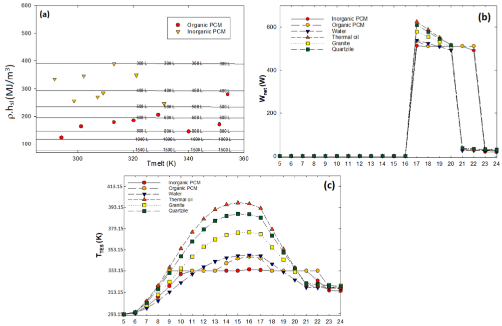
Fig. 2. Characteristic of PCM in full-storage: a) TES capacity, b) W_{\text{net}} , c) T_{\text{TES}}
